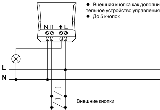
10 А, 3 провода – S5xx525
